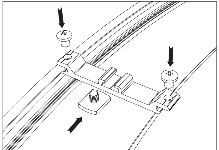
10. install the suspension kits.
