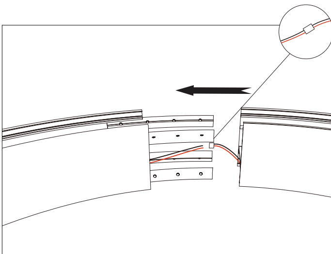
5. Connect the power wires and profiles.
